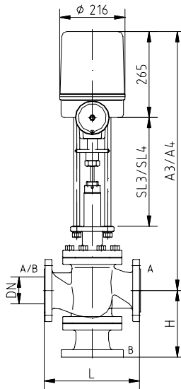
MV 5314 / MV 5324 / MV 5334, #150
