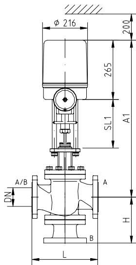
MV 5311 / MV 5321 / MV 5331, #150 / #300
